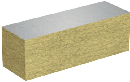
FCFcl Cavity Clad - Horizontal application
