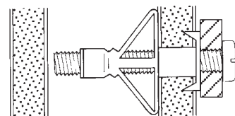
Steel Expanding plasterboard fixing in partition
